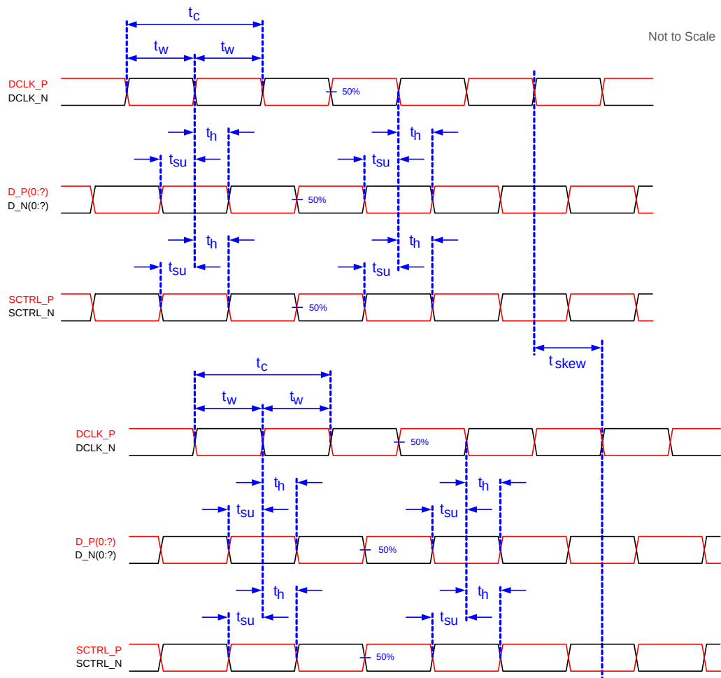
Figure 6. Timing Requirements
